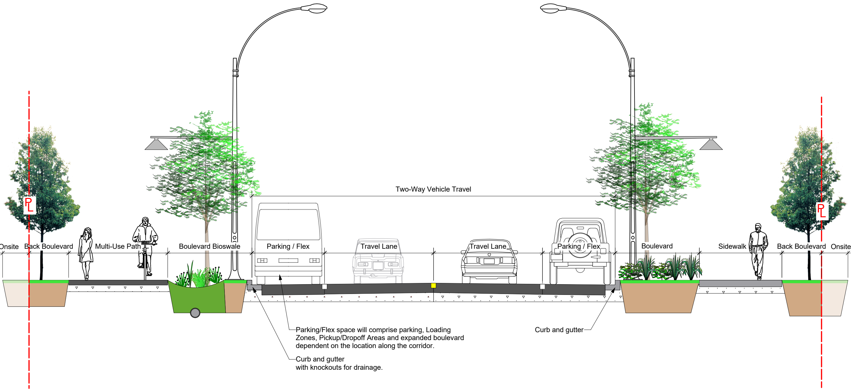
Two Travel Lanes, Two Flex Lanes
