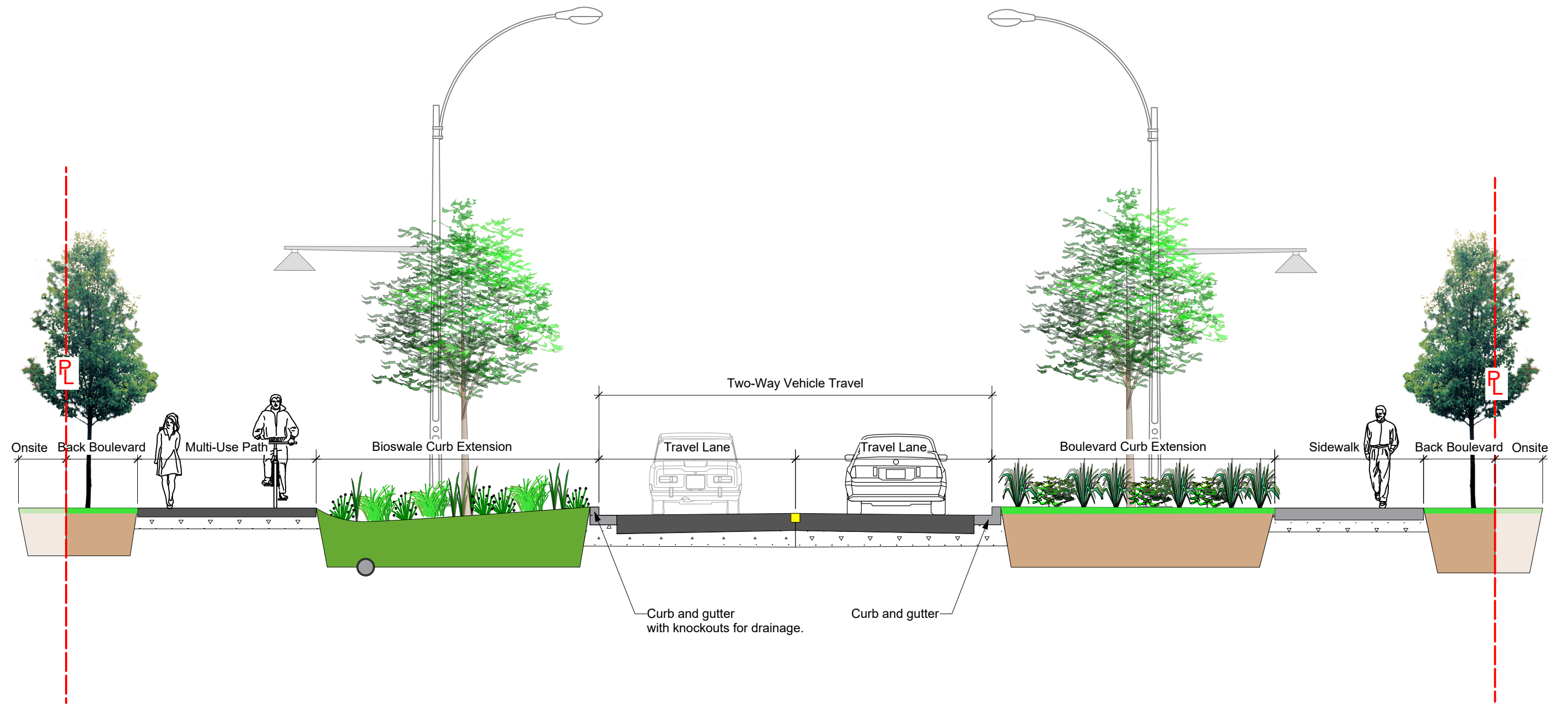
Two Travel Lanes with Curb Extensions
