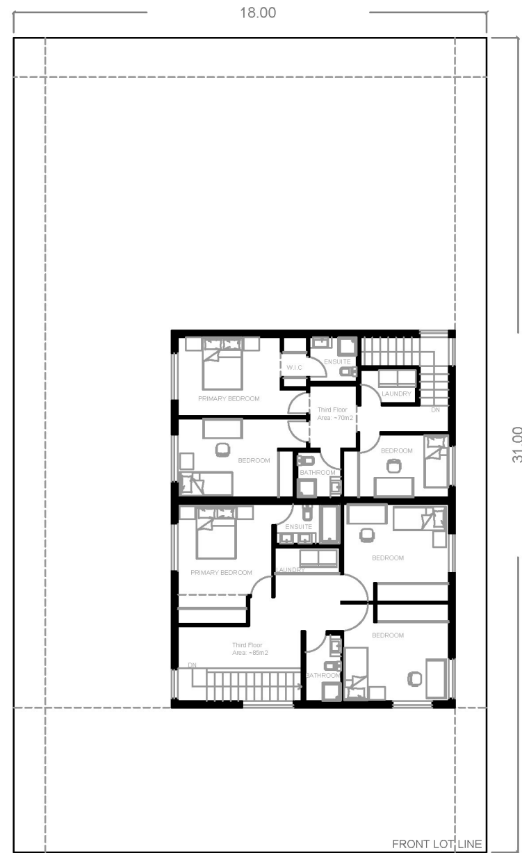
Third Floor Scale: 1:200
