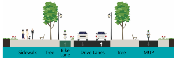
Typical Section, 112 Avenue 26m ROW
